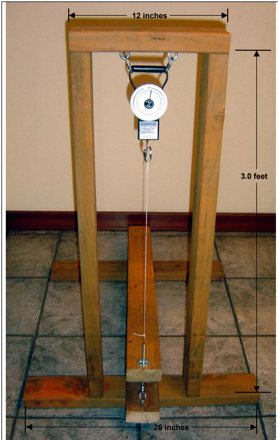
Figure 1. Front view of fiber stress testing apparatus. The test frame can be constructed from standard 2" X 4" pine boards using a handsaw and an electric cordless drill.
