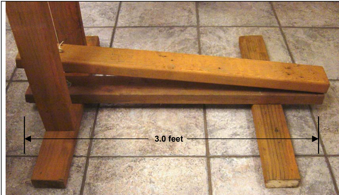
Figure 2. Side view of fiber stress testing apparatus. A simple lever can be constructed using a metal hinge and standard 2" X 4" pine boards.
